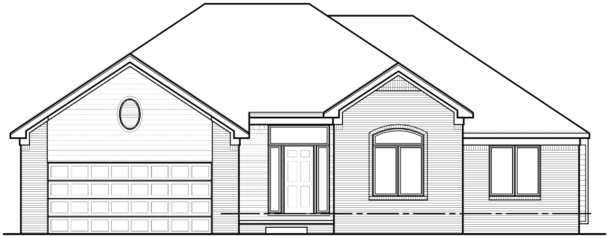
"THE VINNIE" FRONT ELEVATION
